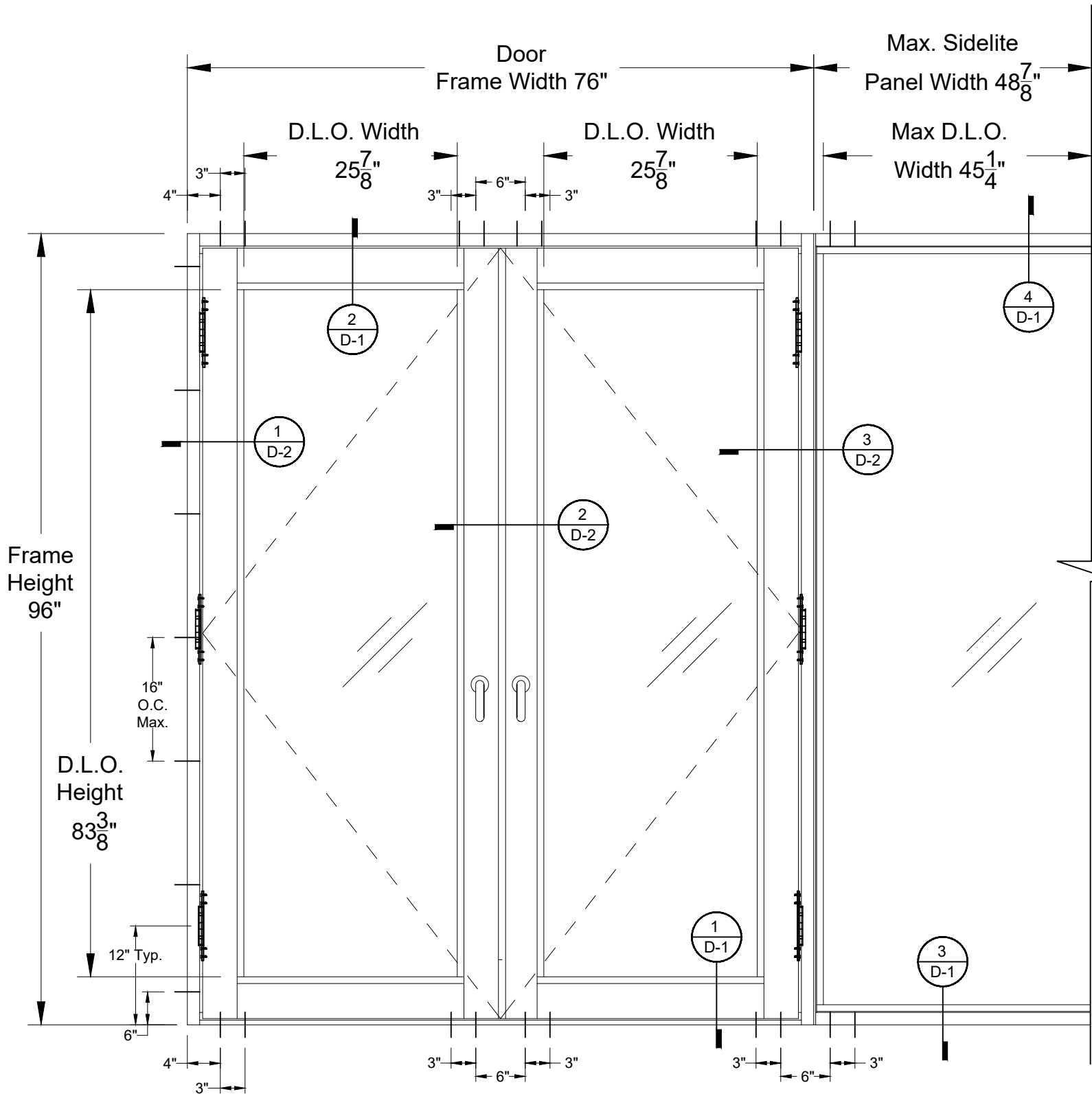
TYP. ELEVATION OF DOUBLE DOOR WITH SIDELITE
