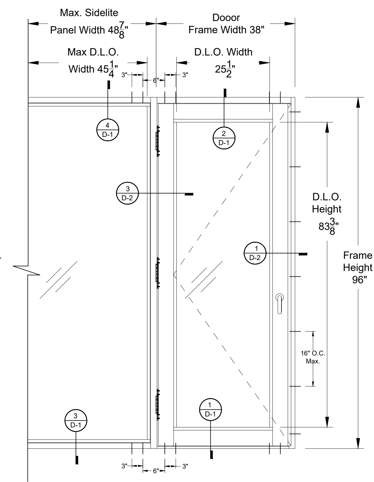
TYP. ELEVATION OF SINGLE DOOR WITH SIDELITE
