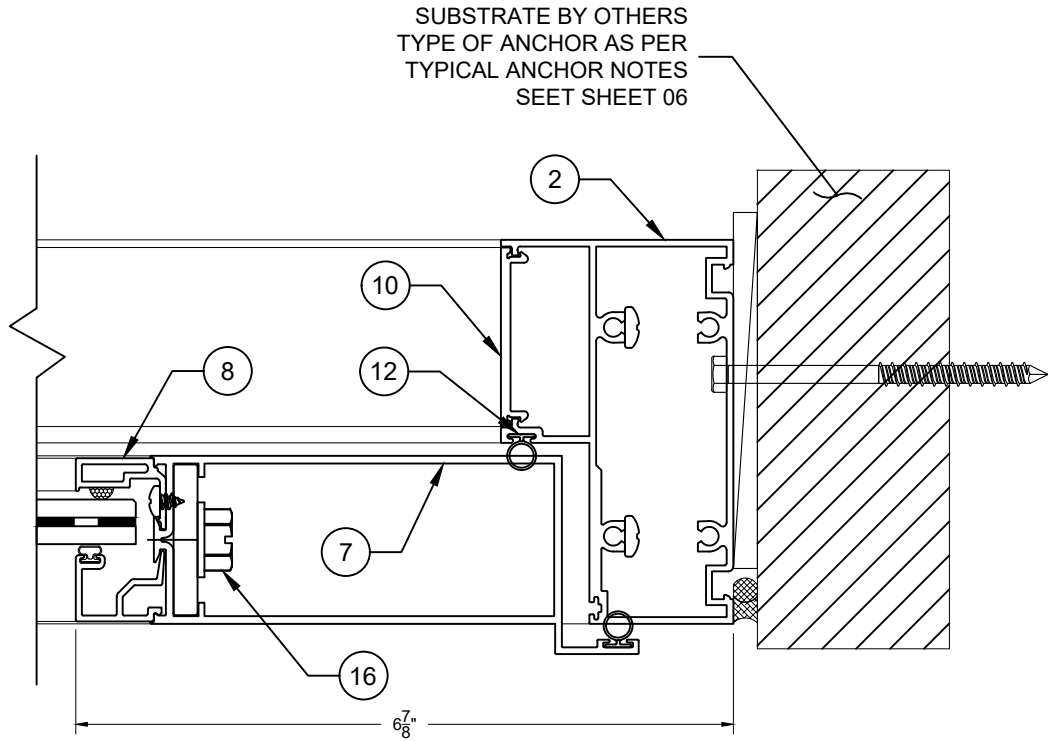
1 Lock Stile Jamb D-3 Scale: As Shown
